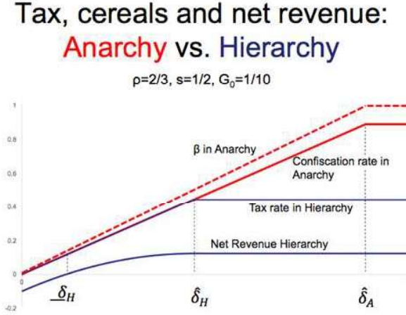
Figure D.1: Tax, cereals and net revenue: Anarchy vs. Hierarchy
