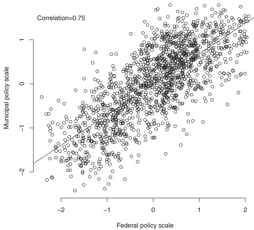
FIGURE 14. Correlations between Municipal and Federal Scales
