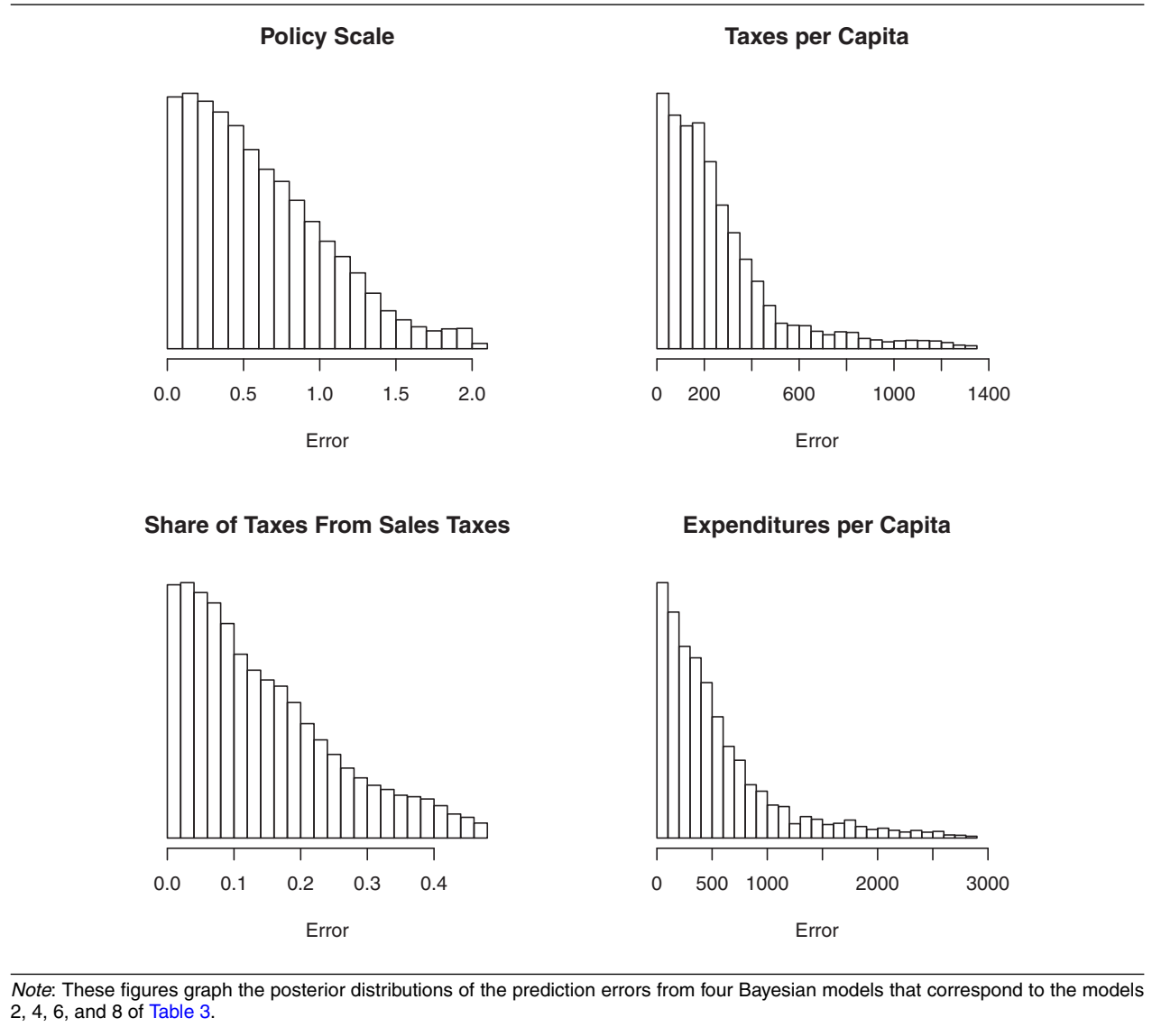
FIGURE 4. Error Distribution of Responsiveness Residuals
